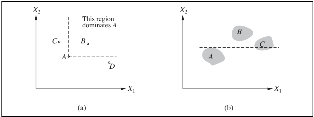
Figure 16.4 Strict dominance. (a) Deterministic: Option A is strictly dominated by B but not by C or D. (b) Uncertain: A is strictly dominated by B but not by C.
